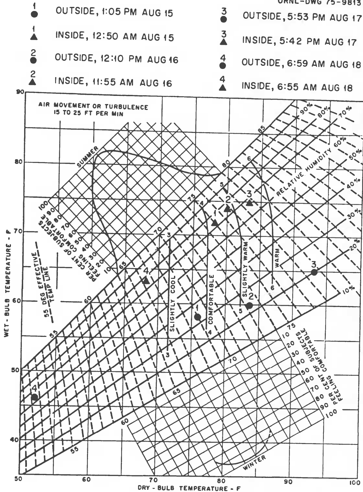
Fig. 4.19. Eight approximately paired temperatures (° F), four outside and four inside the Log-Covered Trench Shelter with seven occupants.
